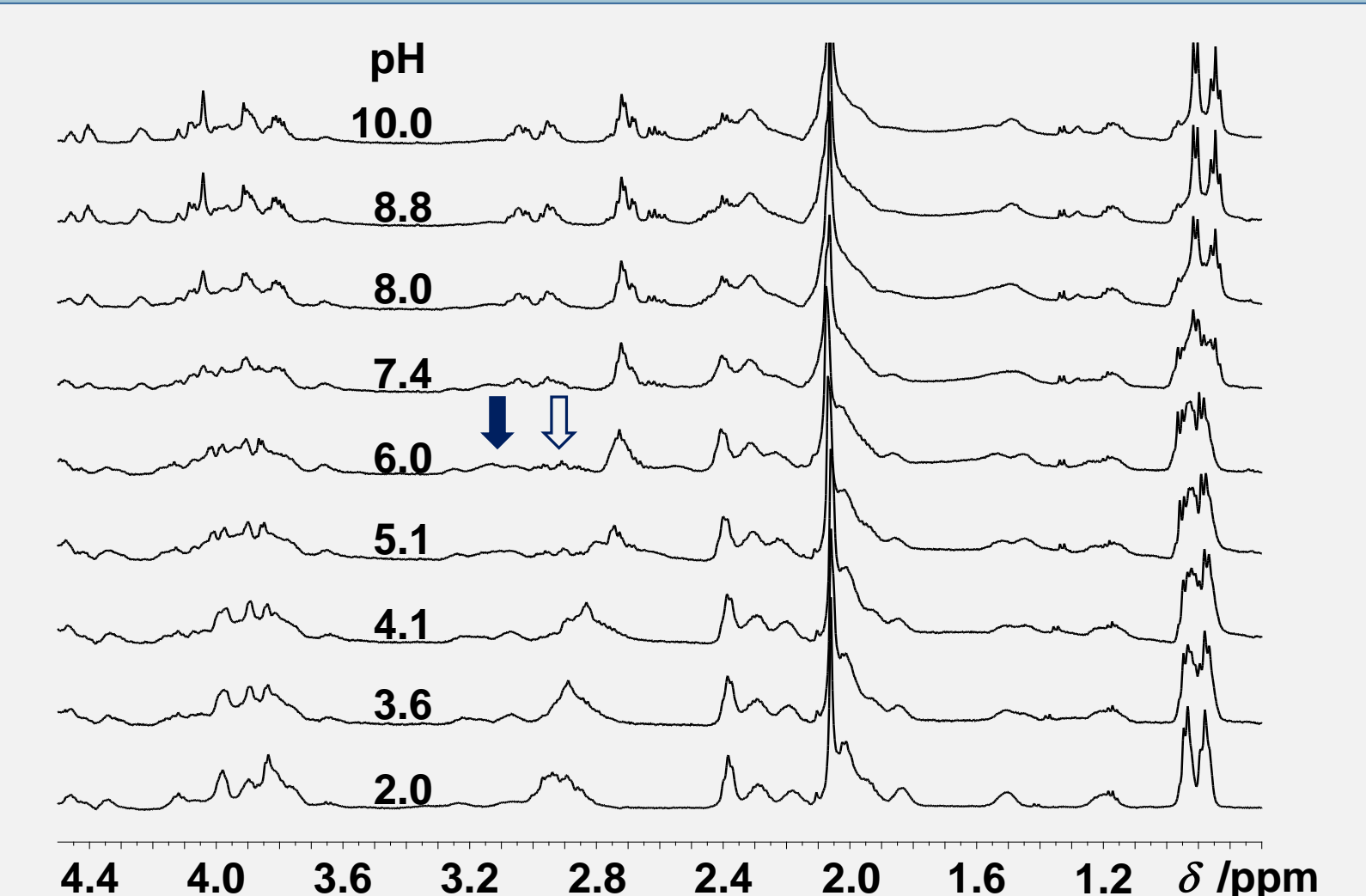
Selected region of the 1 H NMR spectra of the Ag + :PP 1:1 system as a function of pH ( C_{PP} = 1 \times 10^{-3} M). The filled and open arrows point to the bound and unbound Cys C β H 2 signals, respectively.
