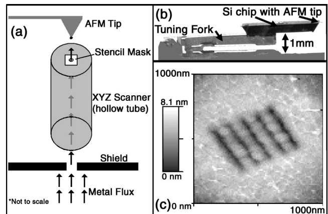
FIG. 1. (a) Schematic diagram of the deposition geometry (not to scale). Metal is deposited from the source, through holes in the stencil membrane, onto the AFM tip. (b) Picture of a commercial AFM tip mounted on a tuning fork used for sensing the tip–surface interaction. (c) AFM image of a pattern of holes in a stencil membrane, acquired prior to deposition.
