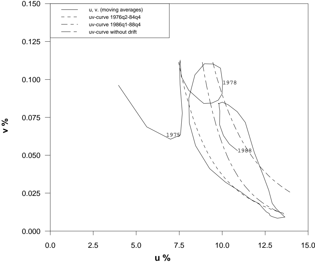
Figure 3: The uv-relations
