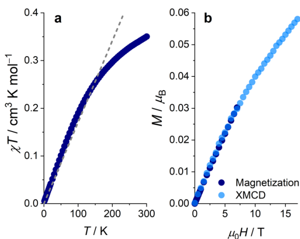
Figure 2. (a) Temperature dependence of the \chi T product ( \chi being the magnetic susceptibility defined as M/\mu_0 H ) over the 1.8–300 K range (0.3 K min^{-1} ) of a polycrystalline sample of 1 obtained with \mu_0 H = 1.0 T. The gray, dashed line is the calculated \chi T product using the model of ref. 13 with a \Gamma_1-\Gamma_4 energy splitting of 1300 cm^{-1} . (b) Field-dependence of the magnetization, M(\mu_0 H) , obtained at 4 K in the 0–7 T range and the scaled field dependence of
