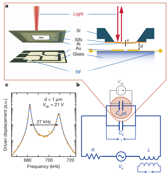
Figure 1 | Optoelectromechanical system. a , A 500- \mu\text{m} -square membrane of Al-coated 30 SiN in vacuum ( <10^{-5} mbar) forms a position-dependent capacitor, C_m(x=0) \approx 0.5 \text{ pF} , with a planar, four-segment gold electrode in the immediate vicinity ( 0.9 \mu\text{m} \lesssim d \lesssim 6 \mu\text{m} ). The membrane electrode's potential is electrically floating. The membrane's displacement is converted into a phase shift of the laser beam reflected from the membrane. b , The membrane capacitor is part of an LC circuit, tuned to the mechanical resonance frequency by means of a tuning capacitor C_0 \approx 80 \text{ pF} (Supplementary Information). A bias voltage, V_{dc} , couples the excitations of the LC circuit to the membrane's motion. The circuit is driven by a voltage V_s , which can be injected through the coupling port 2 or picked up by the inductor from the ambient radio-frequency (RF) radiation. c , For d = 1 \mu\text{m} , the optically observed response of the membrane to a weak excitation of the system shows a split peak due to strong electromechanical coupling. a.u., arbitrary units.
