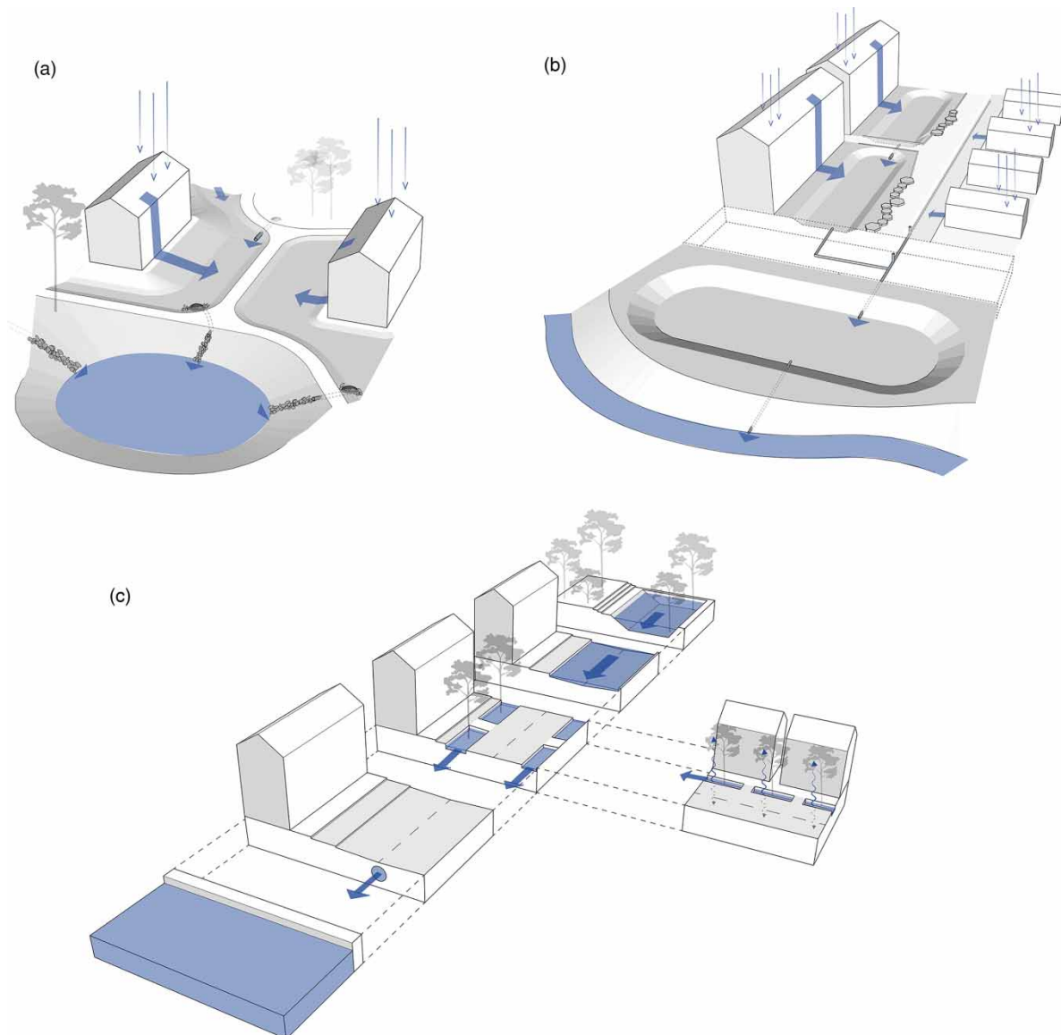
Figure 2 | Illustration of the hydraulic and hydrologic measures used in the three Danish cases. (a) Holmegaardsparken: retention in lawns between raised paths, (b) Kokkedal: Detention in basins and throttled discharge to stream, and (c) Copenhagen Cloudburst Management Plan: Detention in streets, plazas and parks, and discharge to harbour through re-profiled streets and new cloudburst pipes and tunnels. In addition, a number of smaller side streets are to be disconnected permanently from the sewage pipe (illustration to the right, connected with dotted lines to the detention street).
