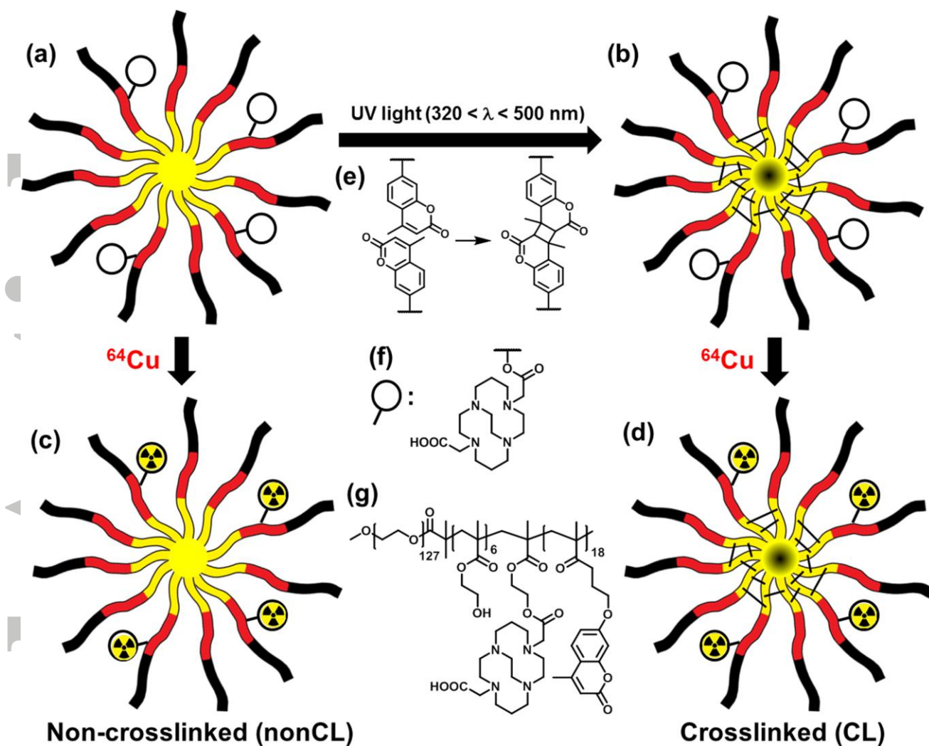
Figure 1. Concept drawing of crosslinking and composition of polymeric micelles. The triblock PEG-PHEMA-PCMA micelle unimers are shown in three colors, with yellow representing the hydrophobic core (PCMA), red the handle domain with CB-TE2A attached (PHEMA) and black the outer hydrophilic PEG domain. (a) Non-crosslinked, non-radiolabeled micelle, (b) Crosslinked, non-radiolabeled micelle, (c) Non-crosslinked micelle, radiolabeled with ^{64}\text{Cu} (nonCL), (d) Crosslinked micelle, radiolabeled with ^{64}\text{Cu} (CL), (e) Photo-induced crosslinking reaction between two 4-methylcoumarin moieties, (f) Structure of the CB-TE2A chelator, (g) Structure of the PEG-PHEMA-PCMA unimer, consisting of 18 coumarin repeats, 7 functionalizable alcohol repeats with one conjugated CB-TE2A, and 127 PEG repeats.
