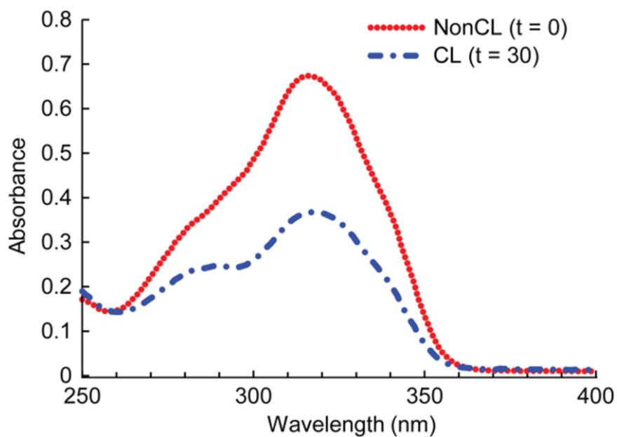
Figure 2. UV chromatograms of polymeric micelles before (NonCL) and after (CL) crosslinking for 30 minutes at 2 \text{ W/cm}^2 (320–500 nm). The degree of crosslinking was measured as the drop in absorbance of the 320 nm maximum from 0.664 to 0.366 giving %CL = 45%.
