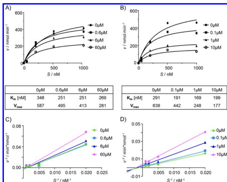
Figure 3. Substrate-dependent inhibition of KDM4C by 4 (A, C) and 23 (B, D). (A, B) The velocity of KDM4C at different inhibitor concentrations is plotted against the substrate concentration, the tables show the respective K_m and V_{max} values. (C, D) Corresponding Lineweaver–Burk plots.
