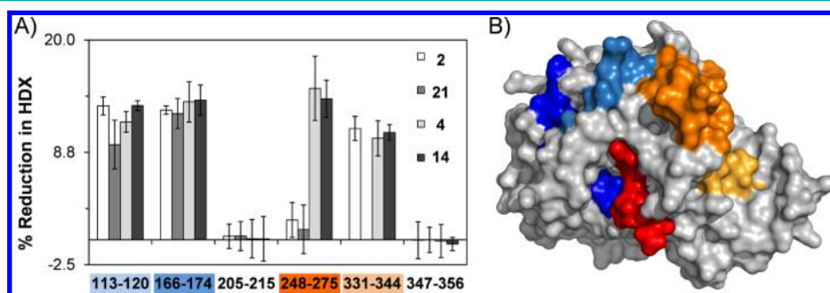
Figure 4. Differential HDX-MS data for KDM4C \pm peptide inhibitors. (A) Histograms showing the percent reduction in HDX for KDM4C residues 113–120, 166–174, 205–215, 248–275, 331–344, and 347–356 by peptides 2, 21, 4, and 14. Values are calculated relative to the measured %D value for free KDM4C ( n = 3 , error bars are standard deviation of the mean). (B) HDX data for the four regions of interest are plotted over the structure of KDM4C (pdb 2XML) with 113–120 highlighted in light blue, 166–174 in blue, 248–275 in orange, and 331–344 in light orange. The histone peptide substrate is shown in red.
