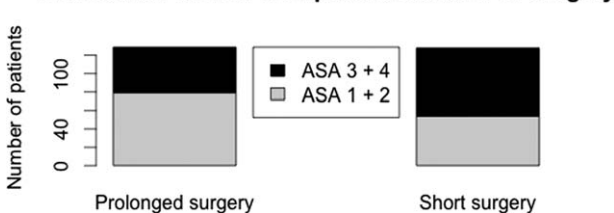
FIGURE 3. Histogram showing the distribution of ASA groups in patients with short and long surgery duration. This shows a selection of low ASA score patients to long surgical time. ASA = American Society of Anesthesiologist.
