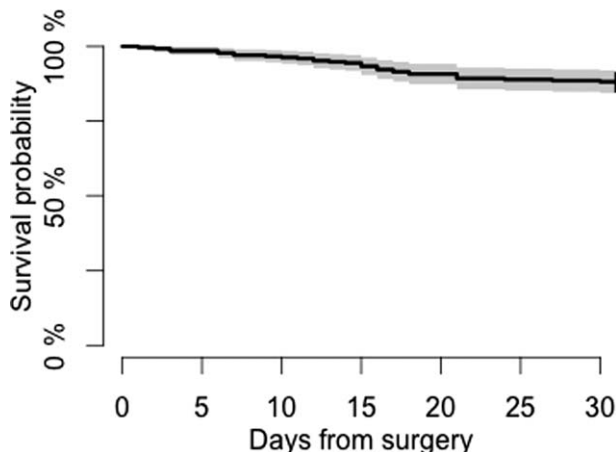
FIGURE 2. Kaplan–Meier survival curves. Thirty-day overall survival with 95% confidence interval.
