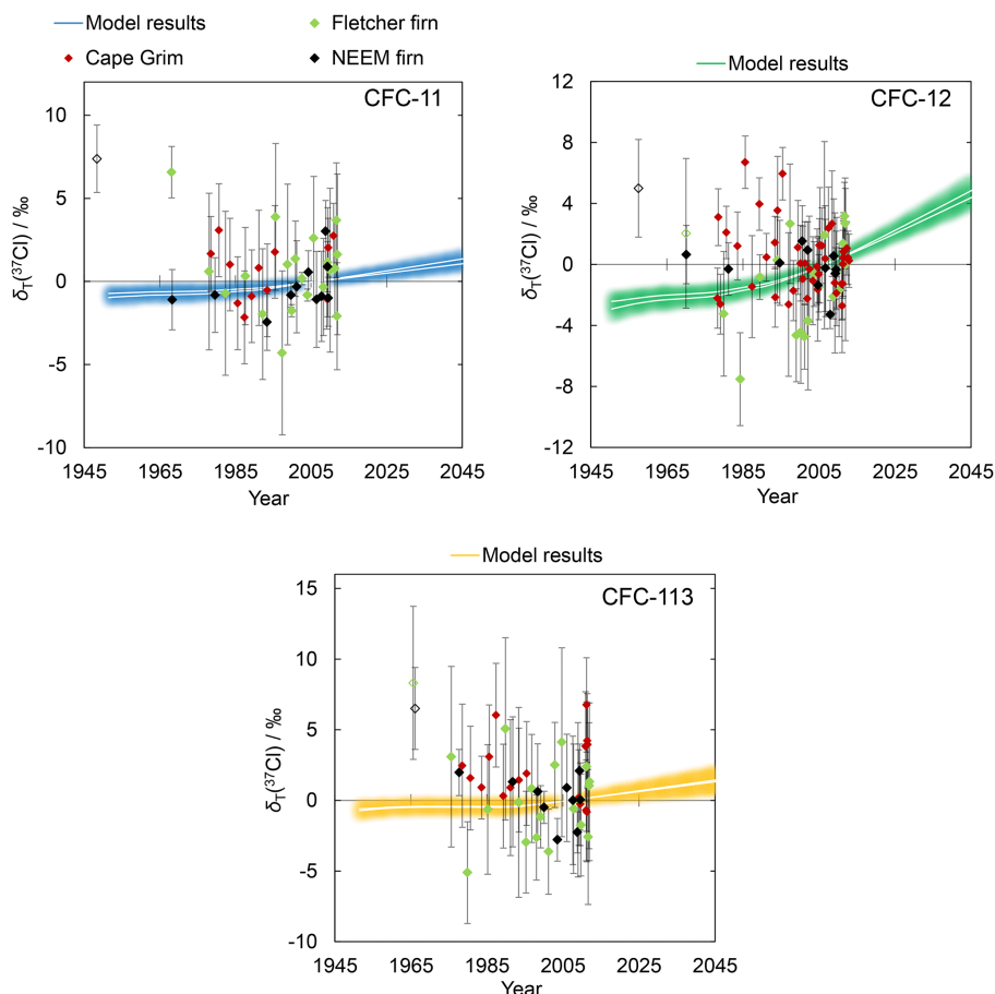
Figure 3. Tropospheric \delta_{\text{T}}(^{37}\text{Cl}) measurements, compared to model predictions. Black diamonds (NEEM firm air), green diamonds (Fletcher Promontory firm air) and red diamonds (Cape Grim air archive) represent the tropospheric chlorine isotope history of CFC-11, CFC-12 and CFC-113. The average repeatability for individual samples was \pm 2.7 ‰ (CFC-11), \pm 2.7 ‰ (CFC-12) and \pm 3.8 ‰ (CFC-113). 1\sigma standard deviation error bars are shown. Open symbols indicate that the measurement was subject to a small correction, based on instrumental nonlinearities (see Supplement). White trend lines represent model estimates of the temporal evolution of \delta_{\text{T}}(^{37}\text{Cl}) values. Two lines are displayed per species, one for each stratosphere–troposphere exchange flux estimate (Holton, 1990; Appenzeller et al., 1996). Blue (CFC-11), green (CFC-12) and orange (CFC-113) shading indicates the model uncertainty envelopes. These uncertainties are based on two independent sources of error: (1) the 1\sigma uncertainty in \varepsilon_{\text{app}} values; (2) the range of most likely lifetime values from SPARC (2013). All \delta values are relative to an air sample collected in 2006 and the model output has been adjusted so that it passes through 0 ‰ at 2006.
