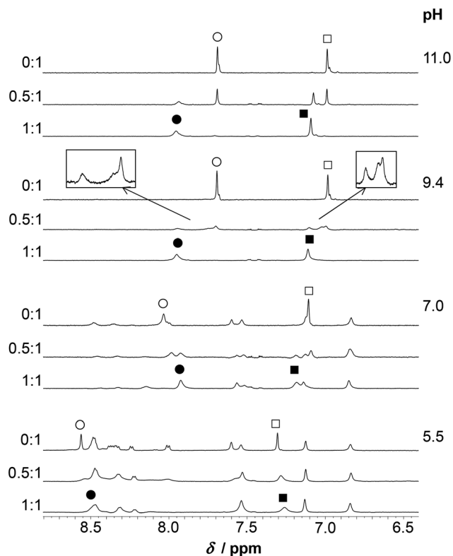
Fig. 10 Aromatic/ ^1\text{H} -N region of the ^1\text{H} NMR spectra of HS recorded in the absence of \text{Zn}^{\text{II}} and in the \text{Zn}^{\text{II}}:\text{HS} 0.5 : 1 and 1 : 1 systems ( \text{H}_2\text{O}/\text{D}_2\text{O} = 90 : 10\% v/v, c_{\text{HS}} = 1.3 \times 10^{-3} M, T = 298 K). The open circle and square symbols show resonances of the non-bound ligand ( \text{C}_{\epsilon 1}\text{H} and \text{C}_{\delta 2}\text{H} , respectively) while the filled symbols mark the same resonances of the bound His residues in the mononuclear species. The regions of \delta = 6.9\text{--}7.15 and 7.4\text{--}8.05 ppm from the \text{Zn}^{\text{II}}:\text{HS} 0.5 : 1 spectrum at pH \sim 9.4 are magnified in the frames.
