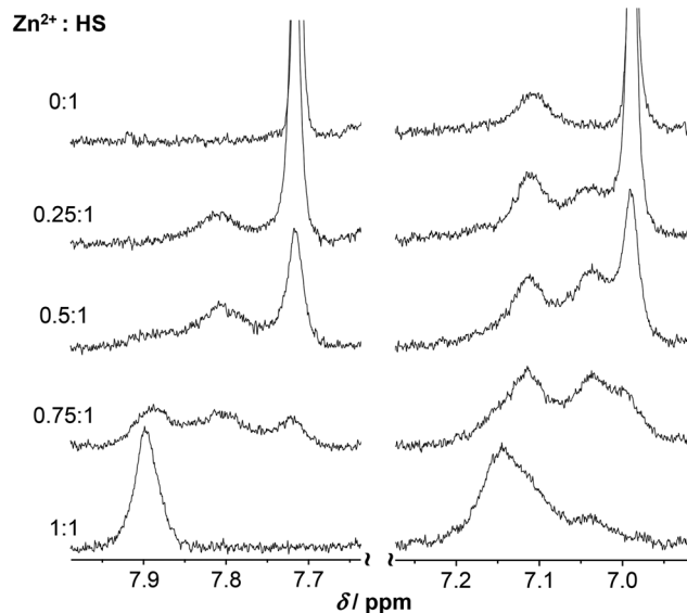
Fig. 11 Part of the ^1\text{H} NMR spectra of HS recorded at pH \sim 8.0 as a function of the metal ion to peptide ratio ( \text{H}_2\text{O}/\text{D}_2\text{O} = 90 : 10\% v/v, c_{\text{HS}} = 1.3 \times 10^{-3} M, T = 298 K). The selected regions reveal changes observed on the \text{C}_{\epsilon 1}\text{H} (left) and \text{C}_{\delta 2}\text{H} (right) resonance of the His-imidazole moiety of the ligand. Note that the peak seen at \delta \sim 7.11 ppm on the free HS spectrum is one of the remaining amide resonances still observable at pH \sim 8.0 .
