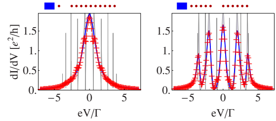
FIG. 4. (Color online) Both panels show the conductance for a chain with ten sites and one weak link with tunnel coupling t_{\text{weak}} = 0.25\Gamma while the other links have t = \Gamma . The weak links are the 1–2 and 5–6 connections for the left/right panel, respectively. The thick (blue) curve is the conductance for kT = 0.1\Gamma , the thin gray curve for kT = 0 while the crosses show the conductance for the chain truncate at the weak link also with kT = 0.1\Gamma . It is clearly seen that the truncated approximation works well, because the chain after the truncations leads to structure barely resolvable, because k_B T is not much smaller than the width ( \approx 0.125 ) of the additional resonances. It should be noted that the situation with only a single deviating link is not the generic situation but it is chosen here to illustrate the point, that the first weak link determines the effective length of the chain.
