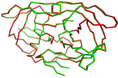
Figure 2. Backbone difference between PyRosetta computed structures of WT-PR and M24. The optimized structures of WT-PR and M24 binding the target peptide were aligned with respect to their \alpha -carbon atoms using PyMol. The backbone of M24 (red) is almost coincident with that of WT-PR (green) with a RMS of 0.227 Å. doi:10.1371/journal.pone.0095833.g002
